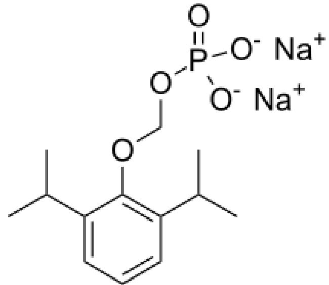
disodium [2,6-di(propan-2-yl)phenoxy]methyl phosphate
